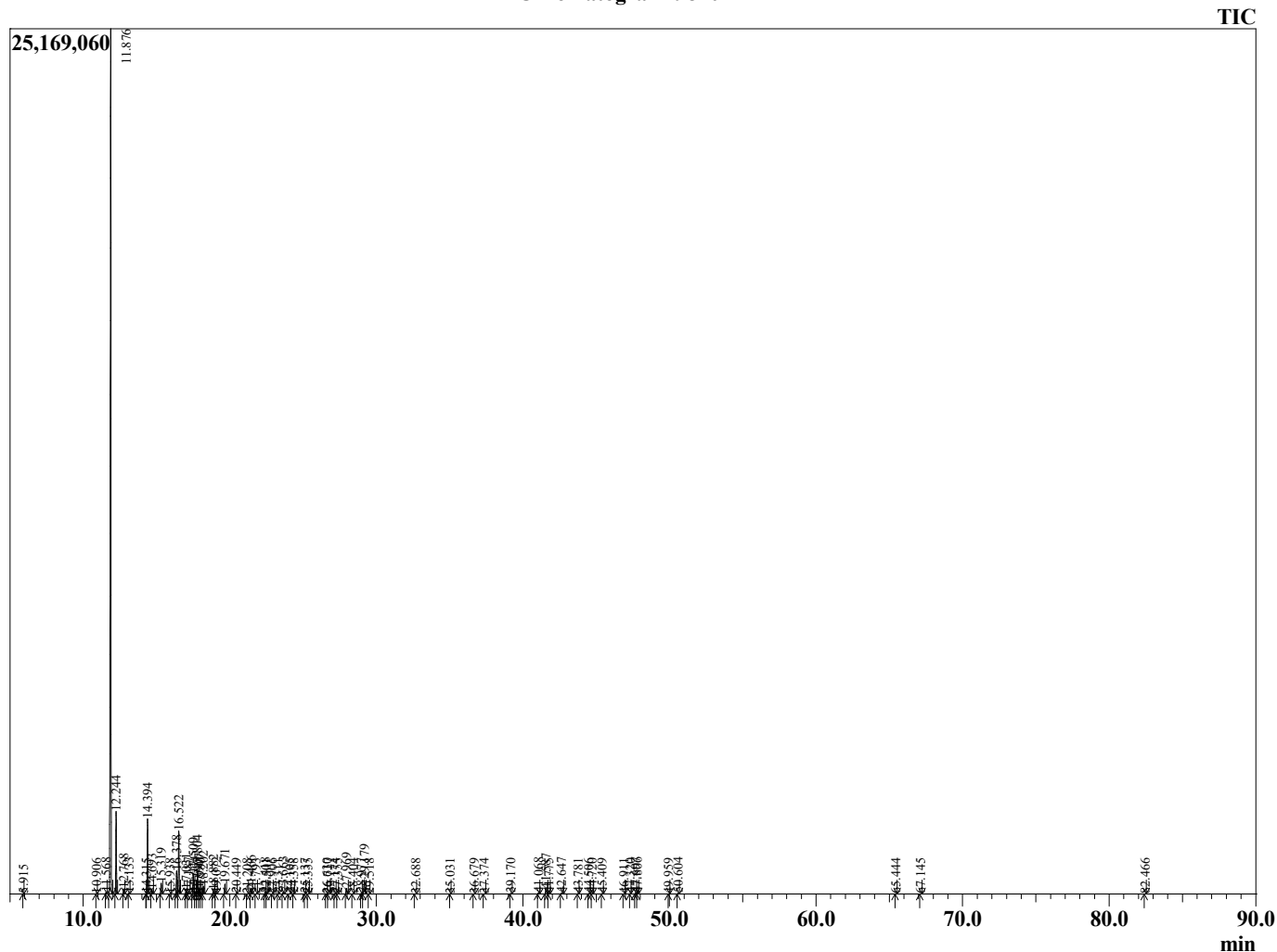
Chromatogram 98401-41
