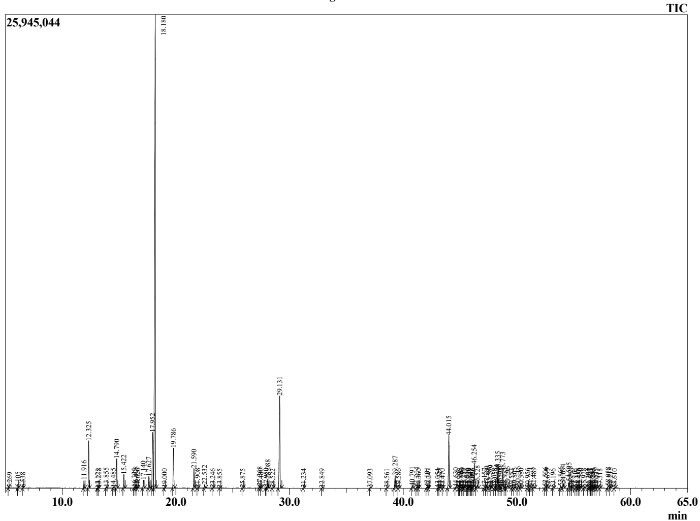
Chromatogram 98401-56
