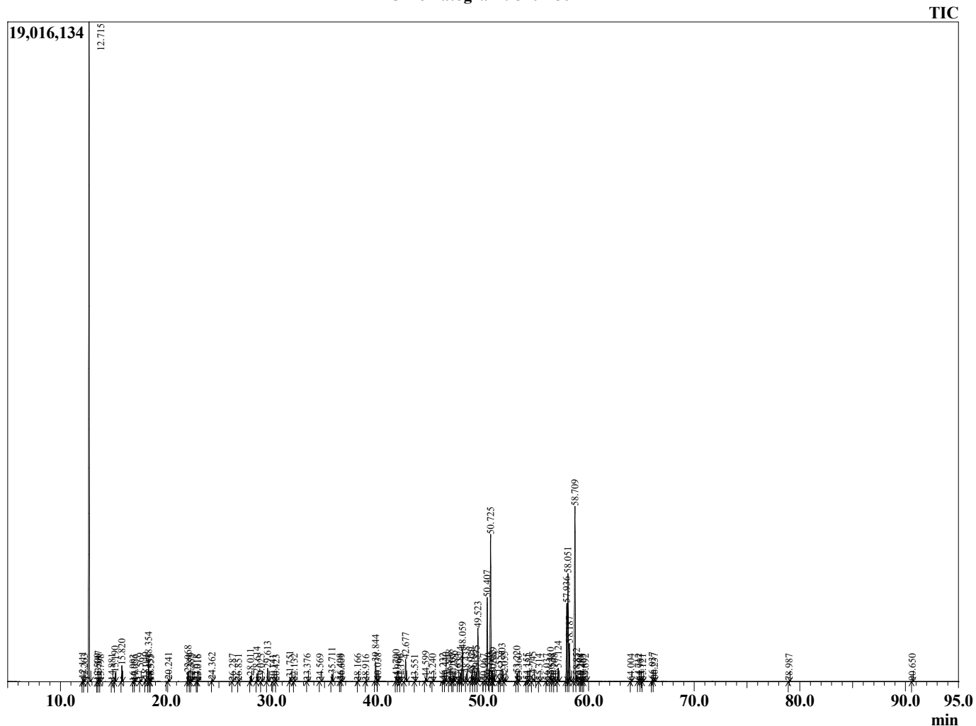
Chromatogram 98401-86
