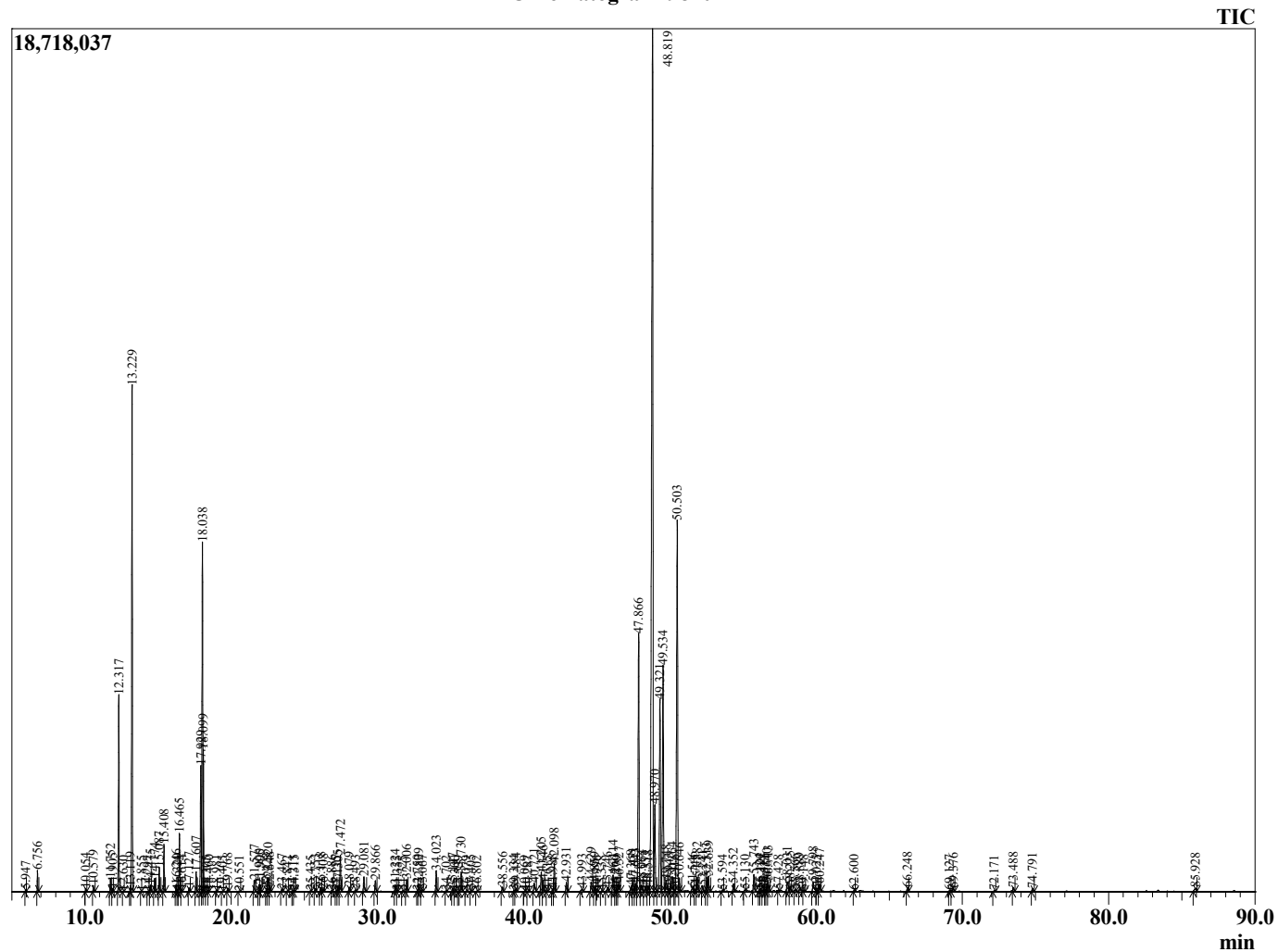
Chromatogram 98401-27
