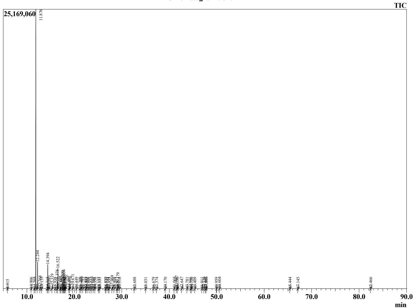
Chromatogram 98401-41
