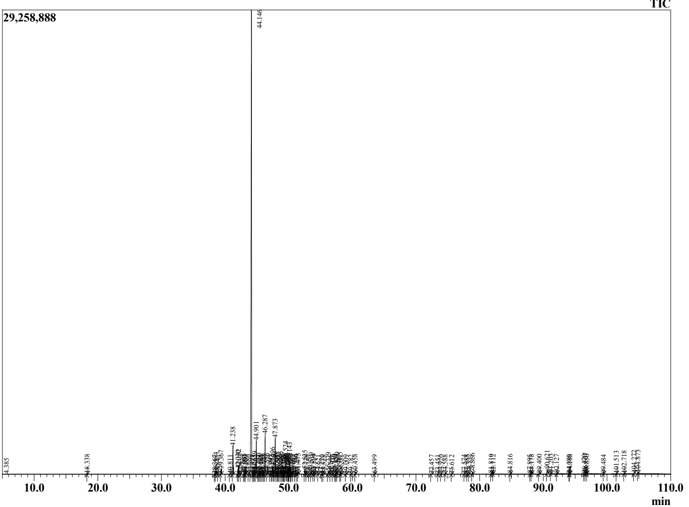
Chromatogram 98401-52
